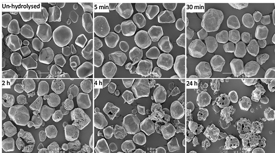
Fig. 5. Electron microscopic images of un-hydrolysed maize starch granules and granule remnant after hydrolysis for 5, 30 min, 2, 4 and 24 h with 0.8 unit FITC-AA conjugate per mg of starch.
